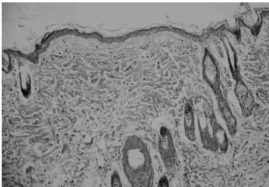
Figure 4B Microscopic photograph ( \times 100 ) of Wistar rat skin after 8 h treatment with 5% eugenol.
